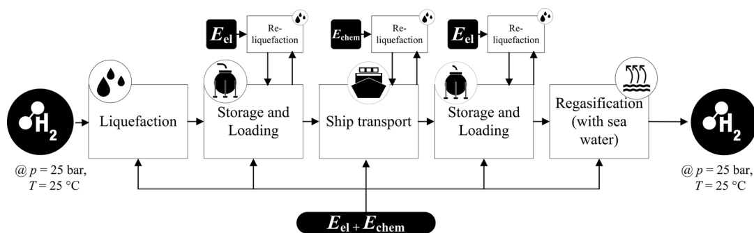
Figure 3. Process chain for hydrogen import option liquid hydrogen (LH 2 ).
